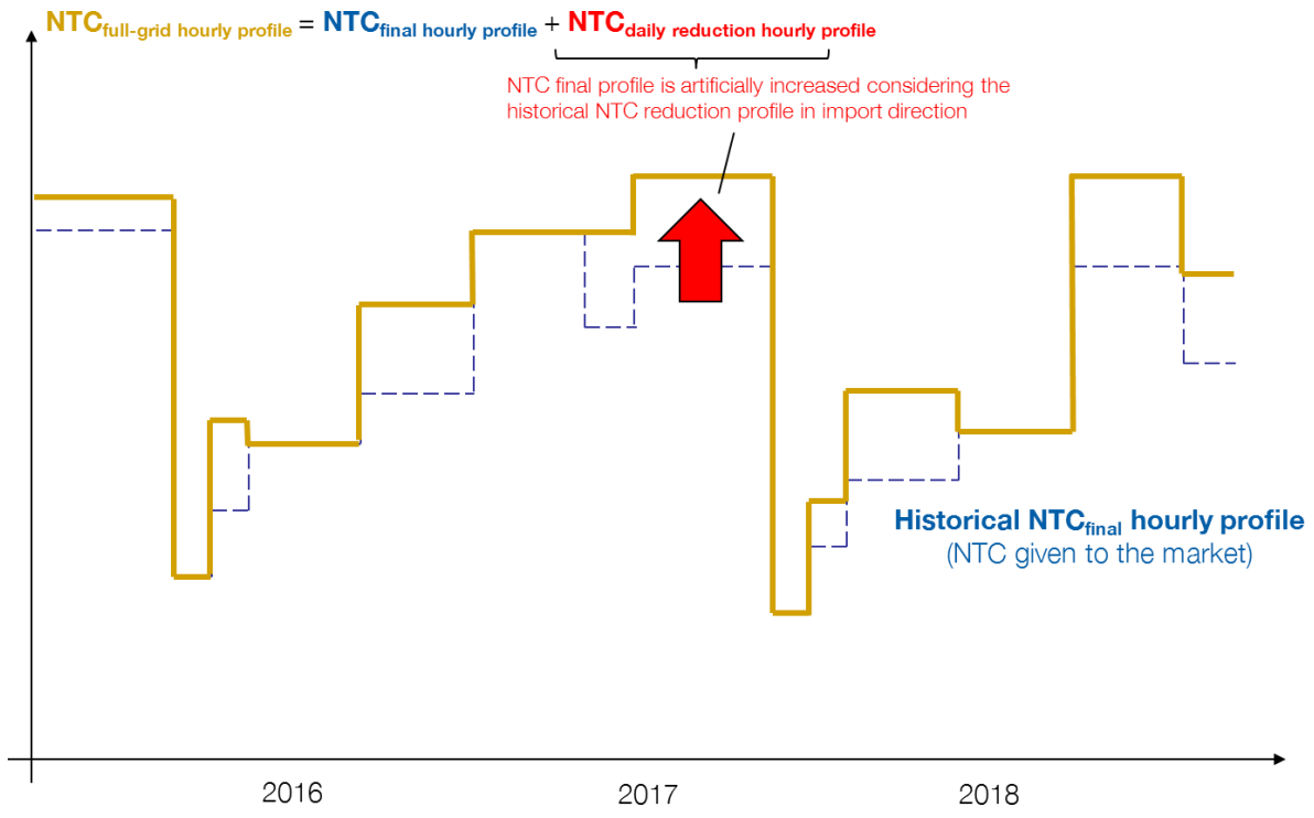
Figure 3: historical full-grid NTC hourly profile computation considering a time window 2016-2018
